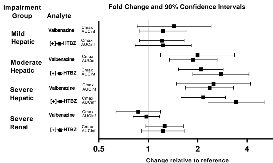
Figure 1: Effects of Hepatic and Severe Renal Impairment on Valbenzazine Pharmacokinetics
